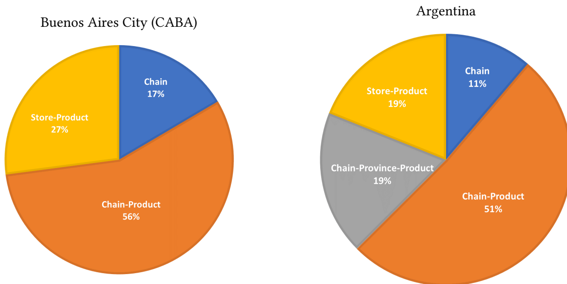
Figure 2: Variance Decomposition of Prices
