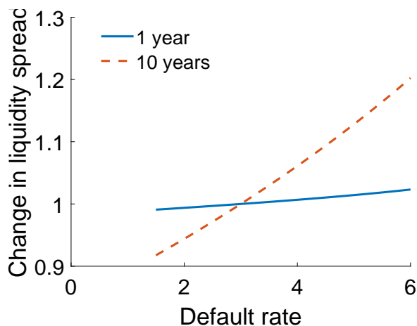
Figure 8: Liquidity-default interactions.
